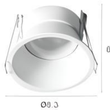
VL-6-W-526 MR16 x 1 ⌀ 7.3 cm
