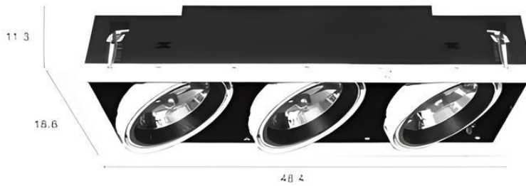
VL-6-W-563-AR111 AR111 x 3 ⌀ 16 x 46 cm.
